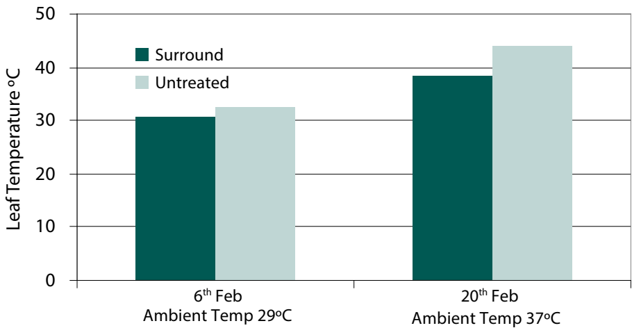
Figure 1. The effect of Surround on grape leaf temperature – Cabernet Sauvignon. University of Melbourne, Dookie Campus. 2005/2006
